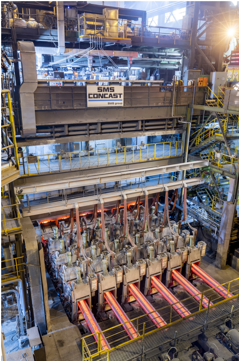
Upgraded SMS Concast bloom caster at Hyundai Pohang, in full production.
